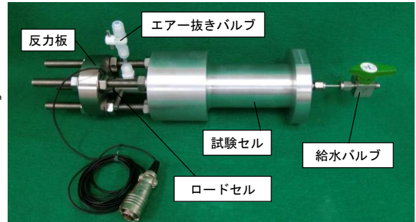
(b) Photo of swelling pressure test apparatus
